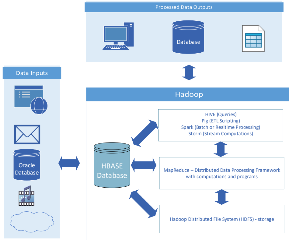
Figure 1: Hadoop Processing
