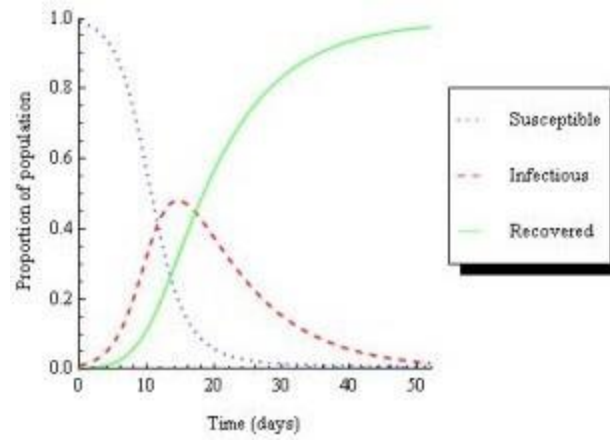
Figure 5: The behavior of SIR model used in Khalil et al. 14
