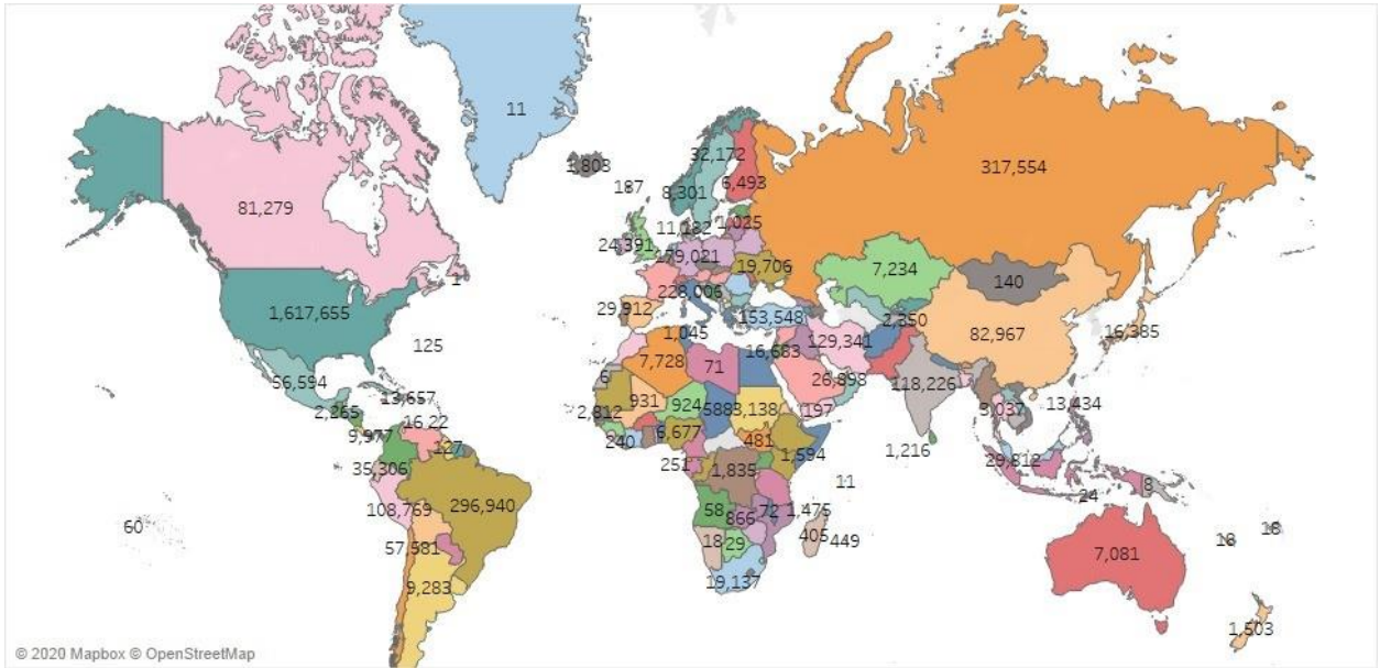
Figure 1: Coronavirus cases distribution around the world May 22, 2020
