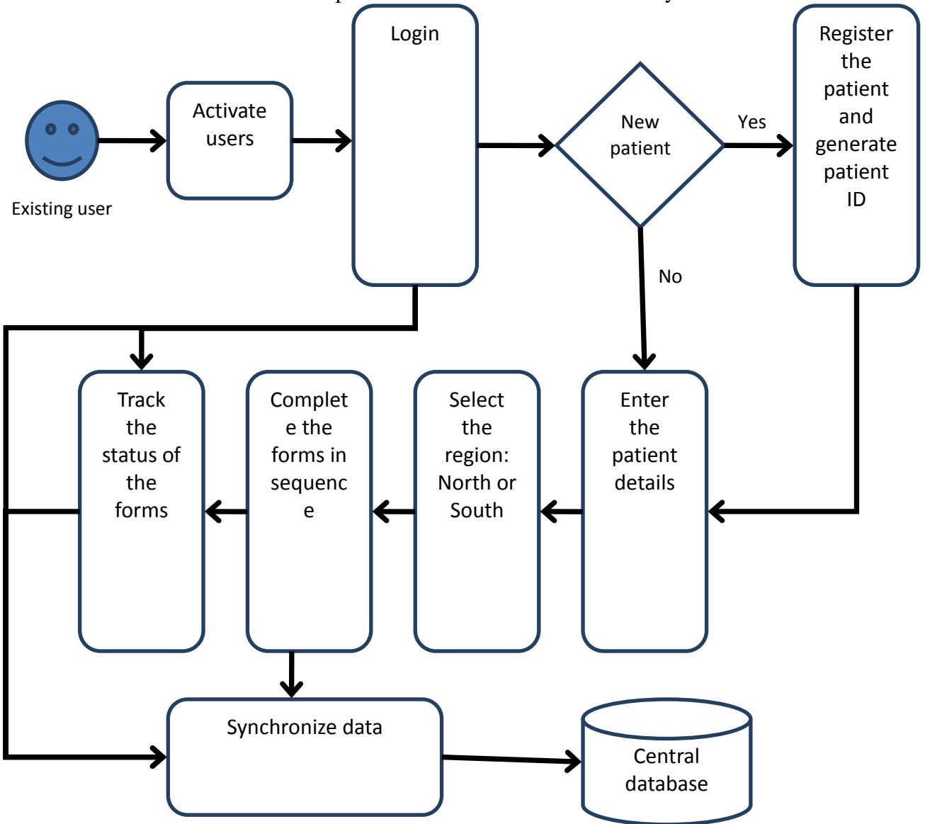
Data Flow for the Stand-alone Desktop-enabled Interactive Surveillance System
